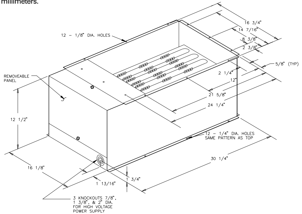
Figure DD-16 — Electric Heater for TWE155 and 200 Air Handlers
